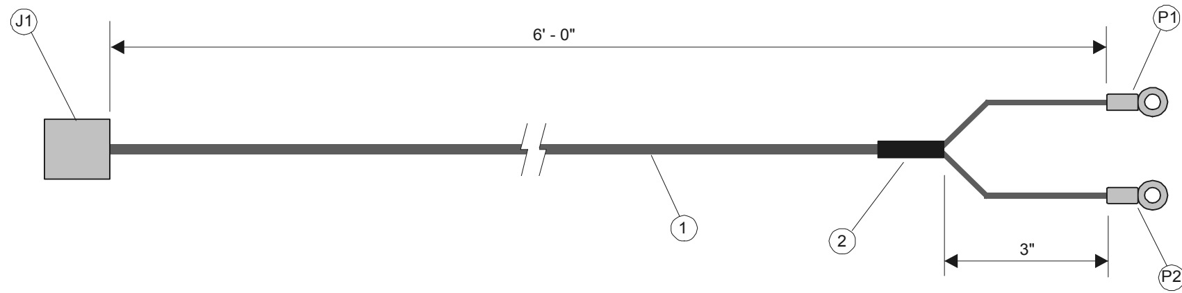
ASSEMBLY DIAGRAM
